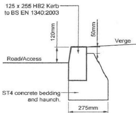
Half Battered Kerb Detail Section B-B
