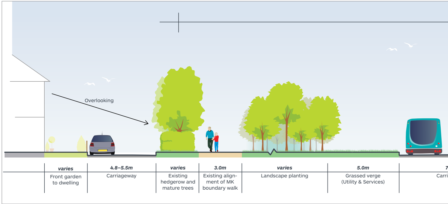
Figure 6.7: Single Carriageway Section - G1
