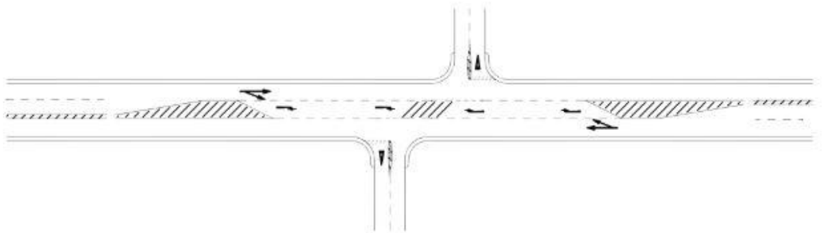
Figure 2.5N1d Staggered junction layouts at changeovers - non-conflicting layout
