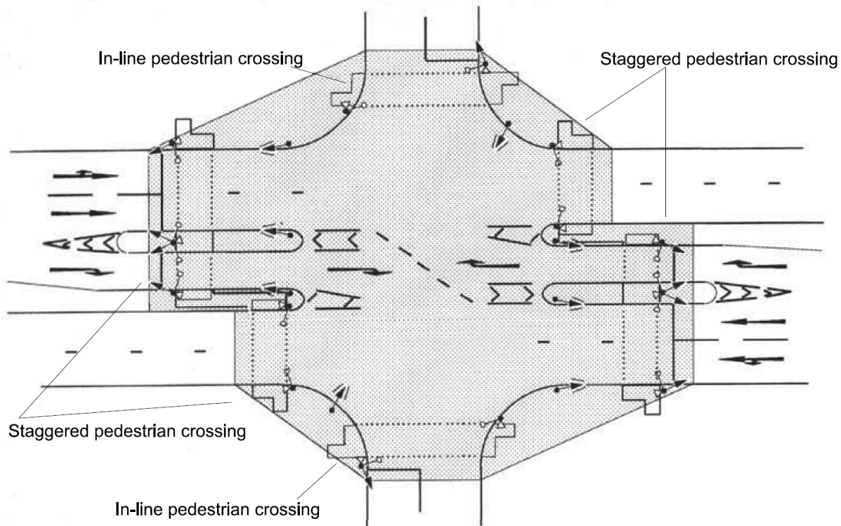
Figure 7.16Nb Offset non-hooking arrangement
