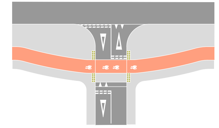
EXAMPLE OF FULL SET BACK (BENT OUT) PRIORITY CROSSING AT THE SIDE ROADS AS FIGURE 10.15 OF LTN1/20
