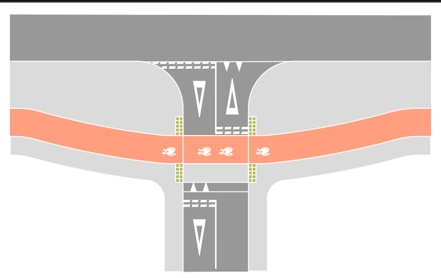
EXAMPLE OF FULL SET BACK (BENT OUT) PRIORITY CROSSING AT THE SIDE ROADS AS FIGURE 10.15 OF LTN1/20
