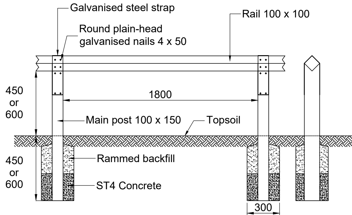
KNEE RAIL FENCE
