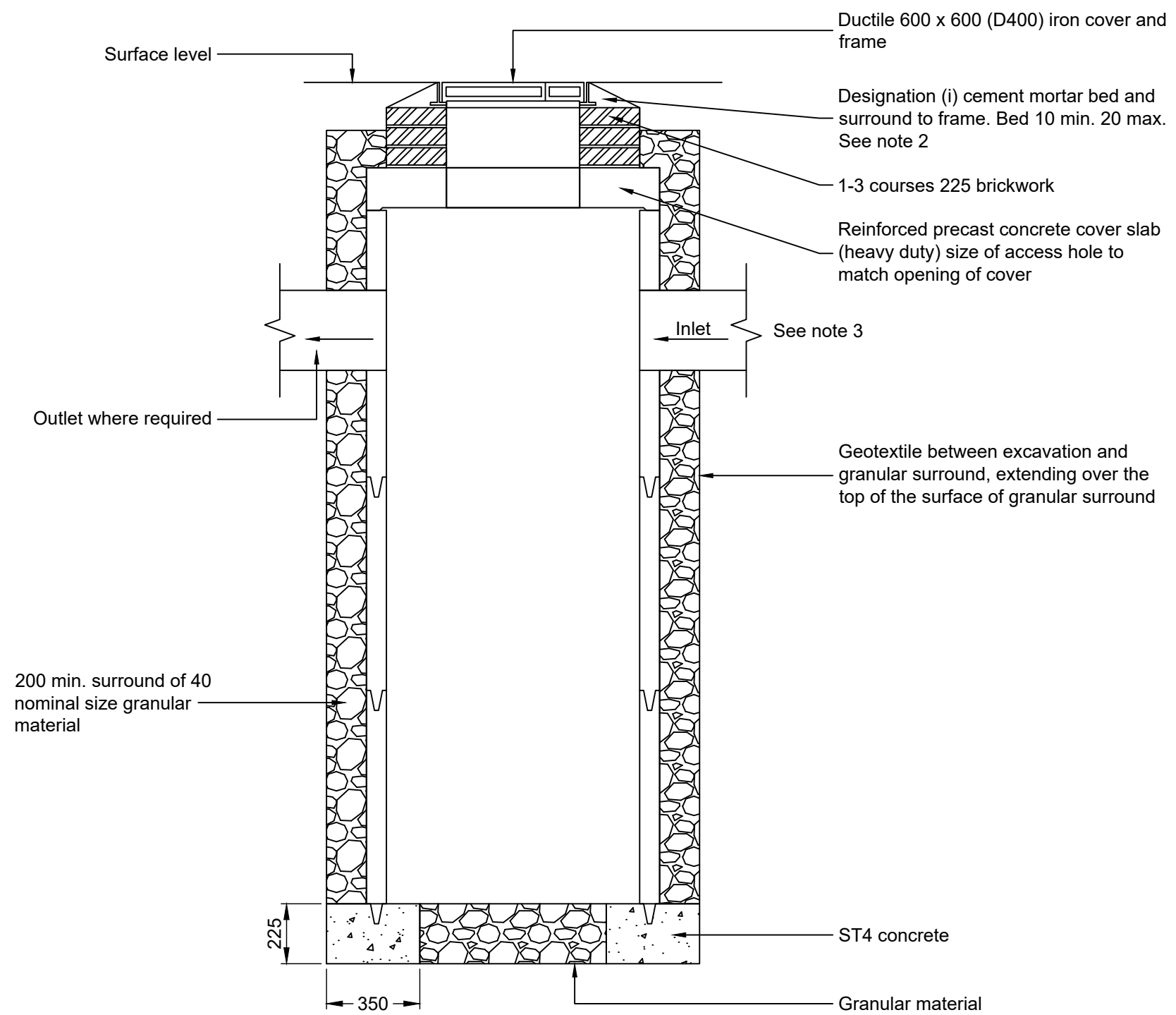
Typical Soakaway Detail
