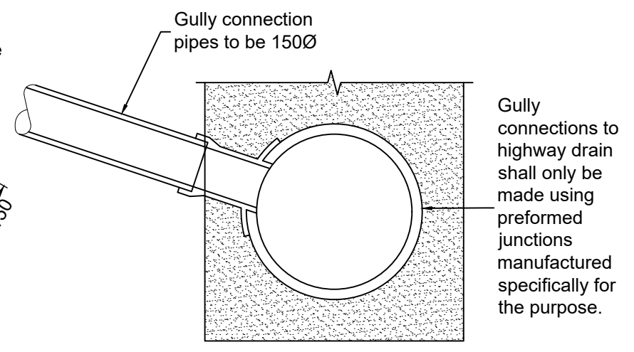
Granular Surround
