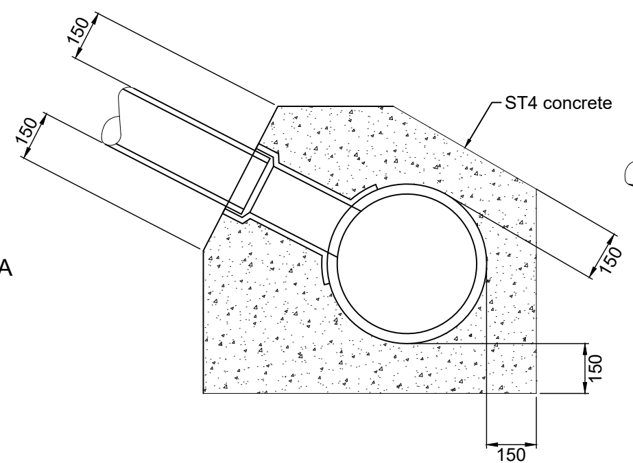
Section A - A Concrete Surround
