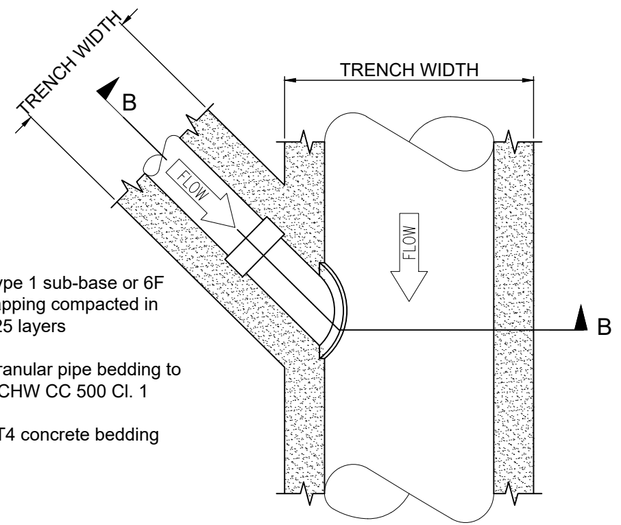
Granular Surround
